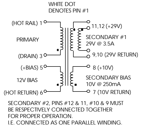
FIGURE 1: SCHEMATIC DIAGRAM
